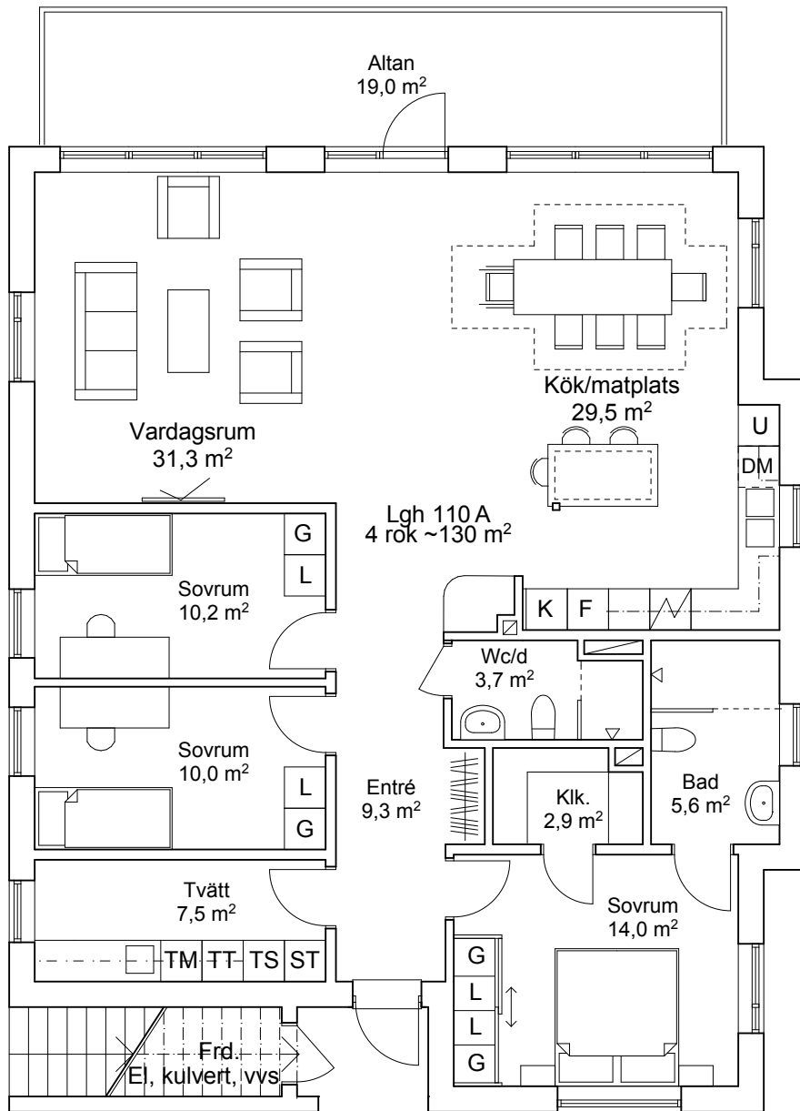
Bottenplan
